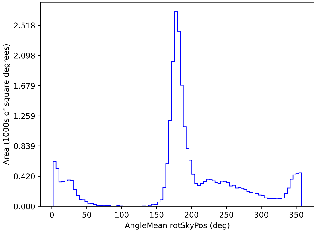
early_u_fpextra2.0_v3.4_10yrs All sky r band: AngleMean rotSkyPos
