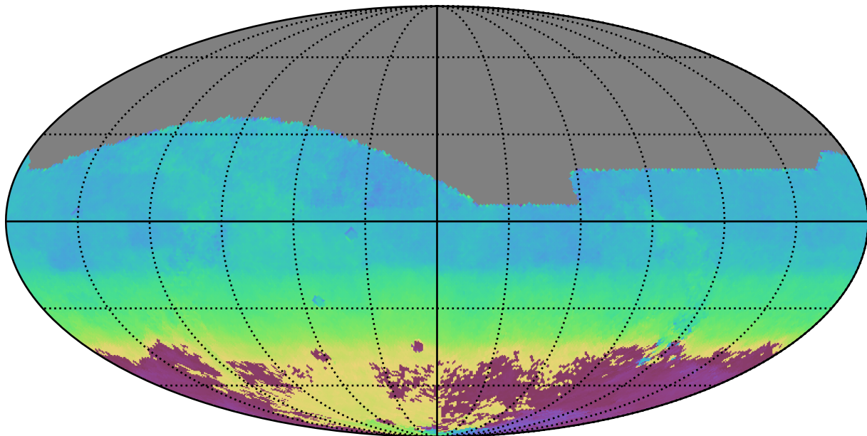
early_u_fpextra2.0_v3.4_10yrs All sky i band: AngleMean rotSkyPos
