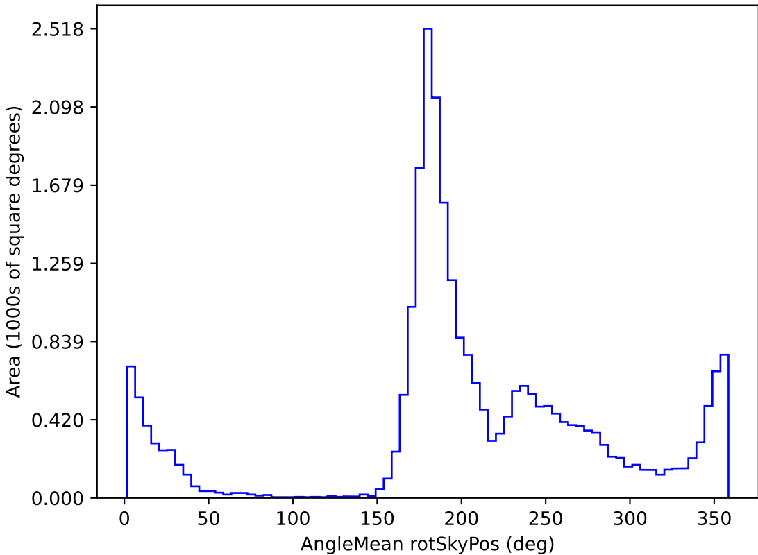
early_u_fpextra2.0_v3.4_10yrs All sky i band: AngleMean rotSkyPos
