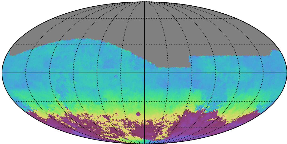
early_u_fpextra2.0_v3.4_10yrs All sky g band: AngleMean rotSkyPos
