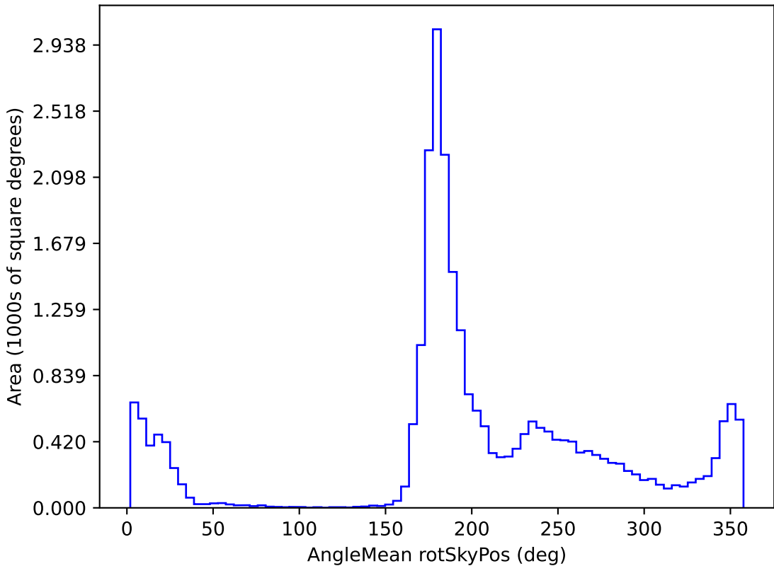
early_u_fpextra2.0_v3.4_10yrs All sky all bands: AngleMean rotSkyPos
