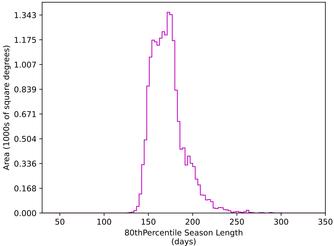
early_u_fpextra2.0_v3.4_10yrs WFD z band: 80thPercentile Season Length
