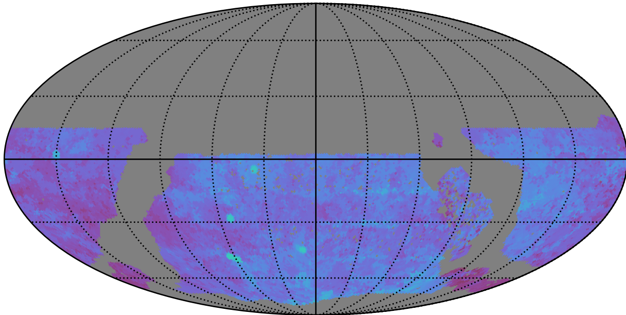
early_u_fpextra2.0_v3.4_10yrs WFD u band: 80thPercentile Season Length
