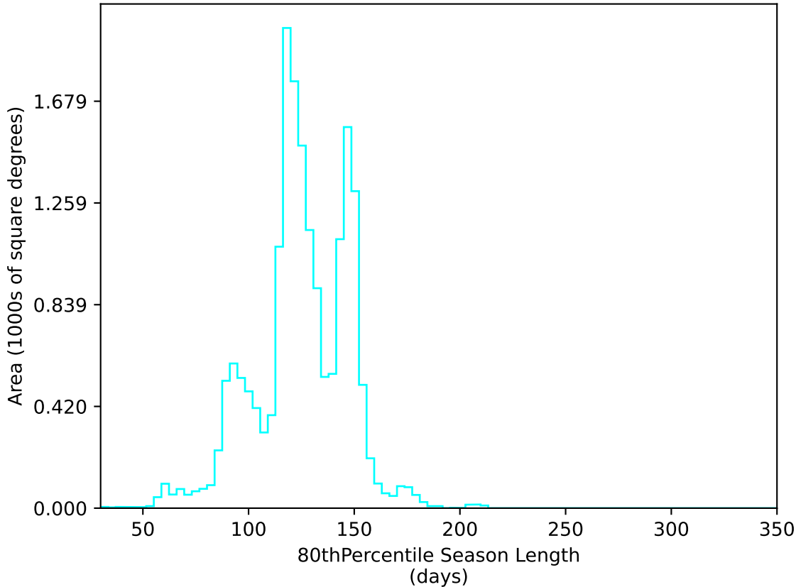
early_u_fpextra2.0_v3.4_10yrs WFD u band: 80thPercentile Season Length
