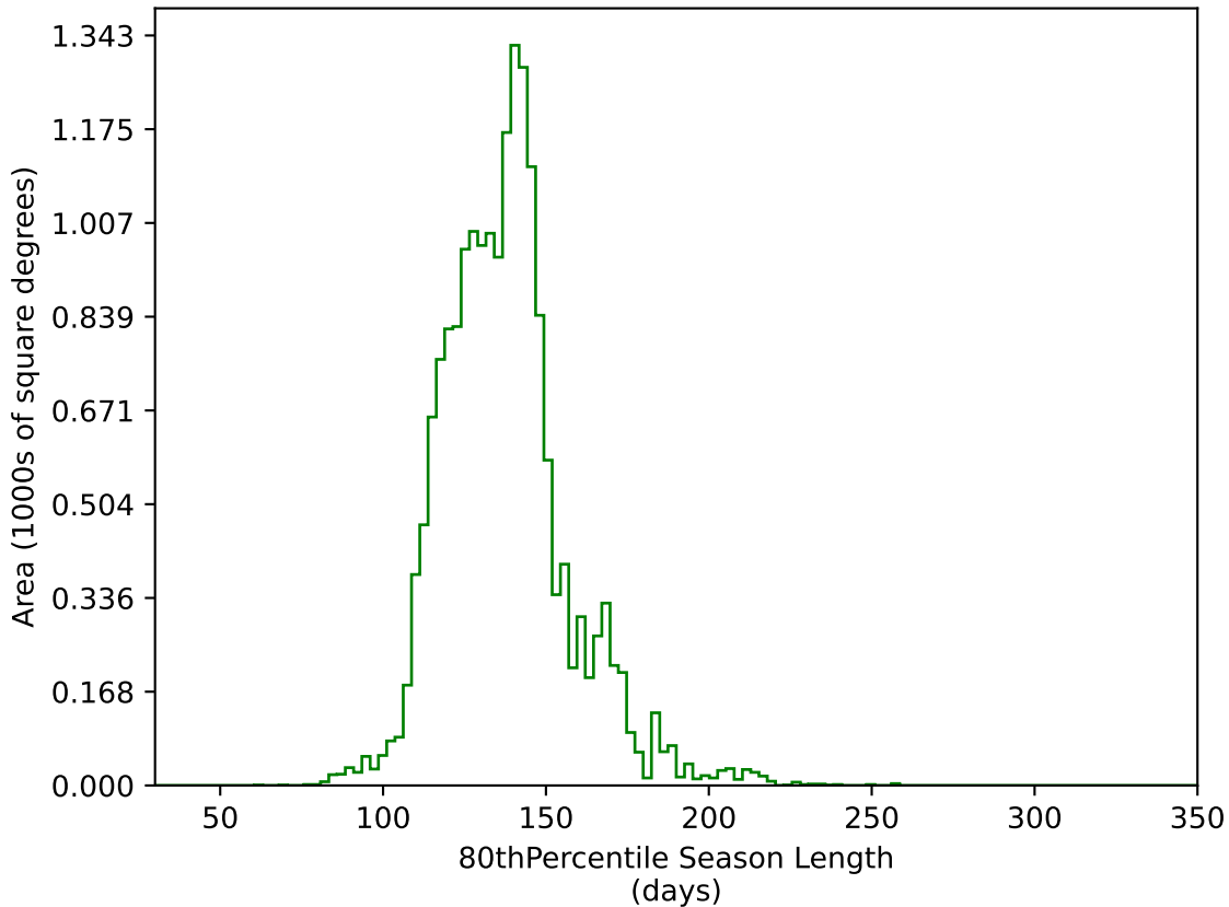
early_u_fpextra2.0_v3.4_10yrs WFD g band: 80thPercentile Season Length
