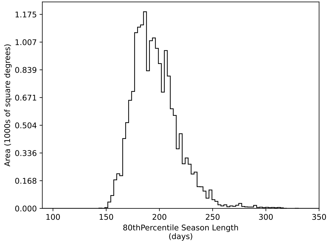
early_u_fpextra2.0_v3.4_10yrs WFD all bands: 80thPercentile Season Length
