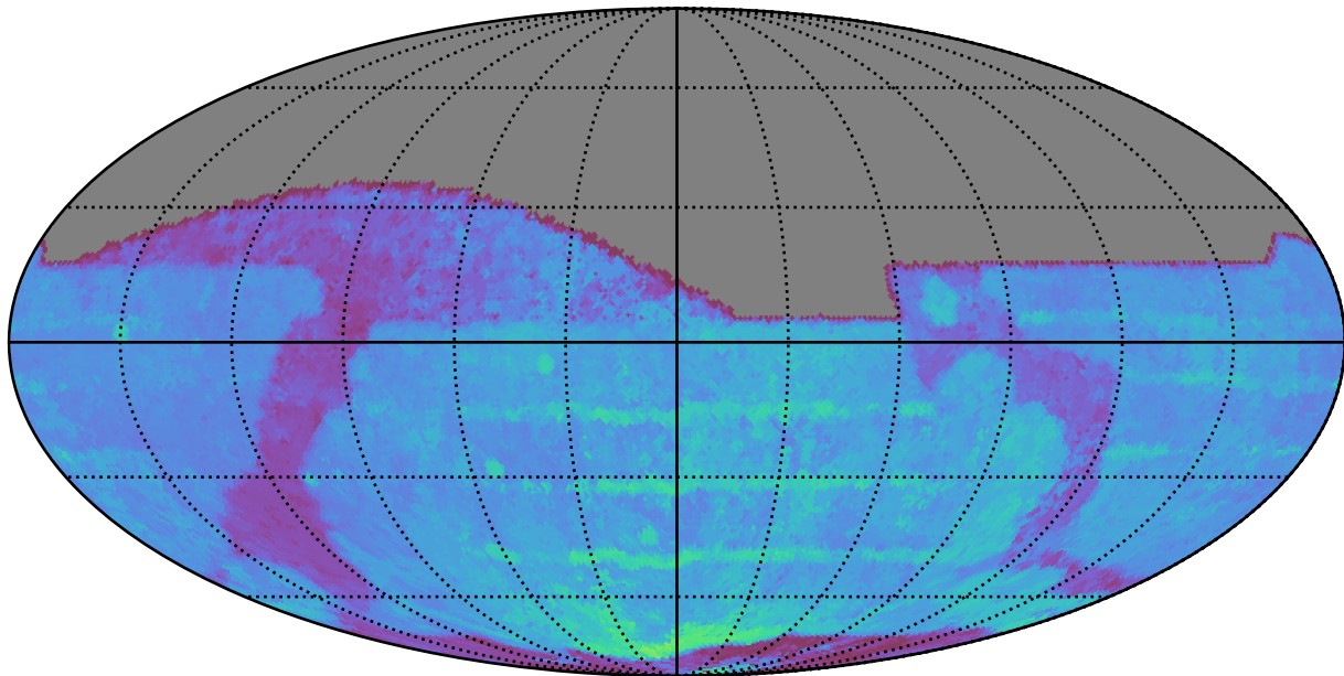
early_u_fpextra2.0_v3.4_10yrs All sky z band: 80thPercentile Season Length
