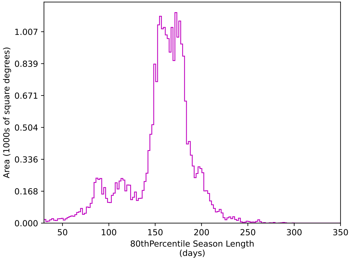
early_u_fpextra2.0_v3.4_10yrs All sky z band: 80thPercentile Season Length
