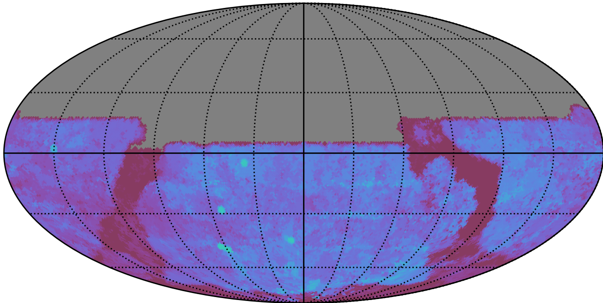
early_u_fpextra2.0_v3.4_10yrs All sky u band: 80thPercentile Season Length
