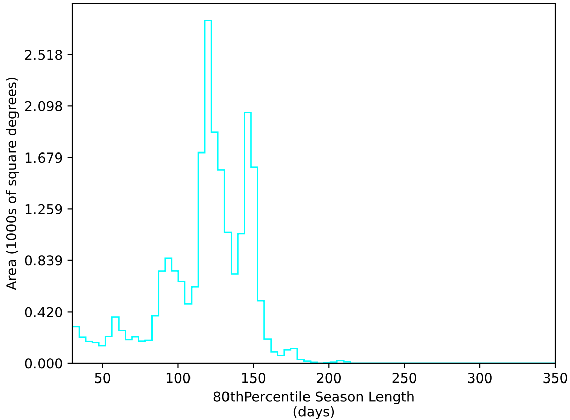
early_u_fpextra2.0_v3.4_10yrs All sky u band: 80thPercentile Season Length
