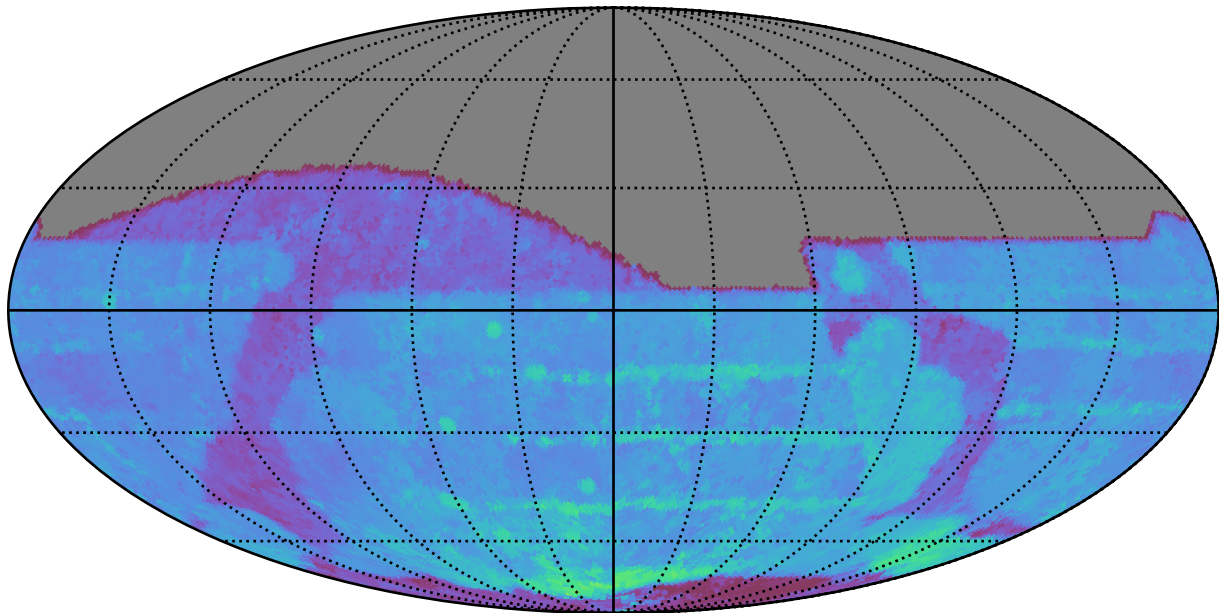
early_u_fpextra2.0_v3.4_10yrs All sky r band: 80thPercentile Season Length
