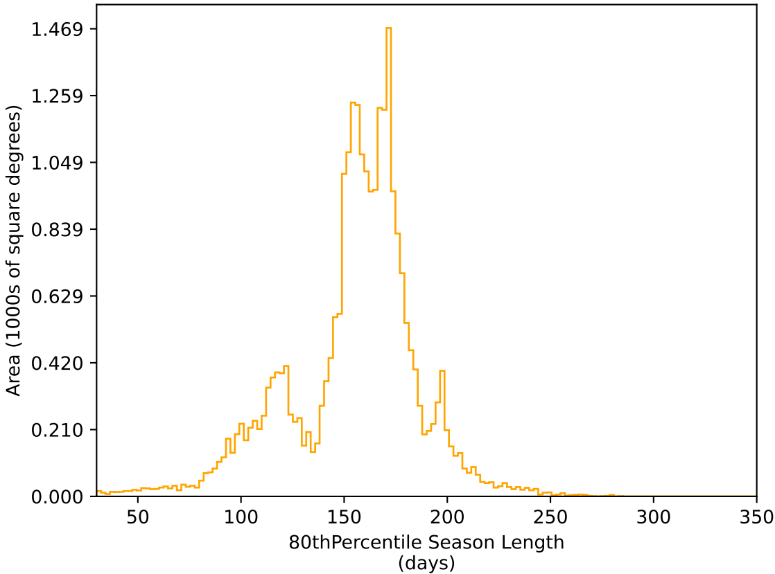
early_u_fpextra2.0_v3.4_10yrs All sky r band: 80thPercentile Season Length
