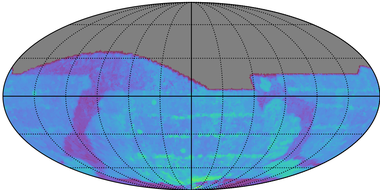
early_u_fpextra2.0_v3.4_10yrs All sky i band: 80thPercentile Season Length
