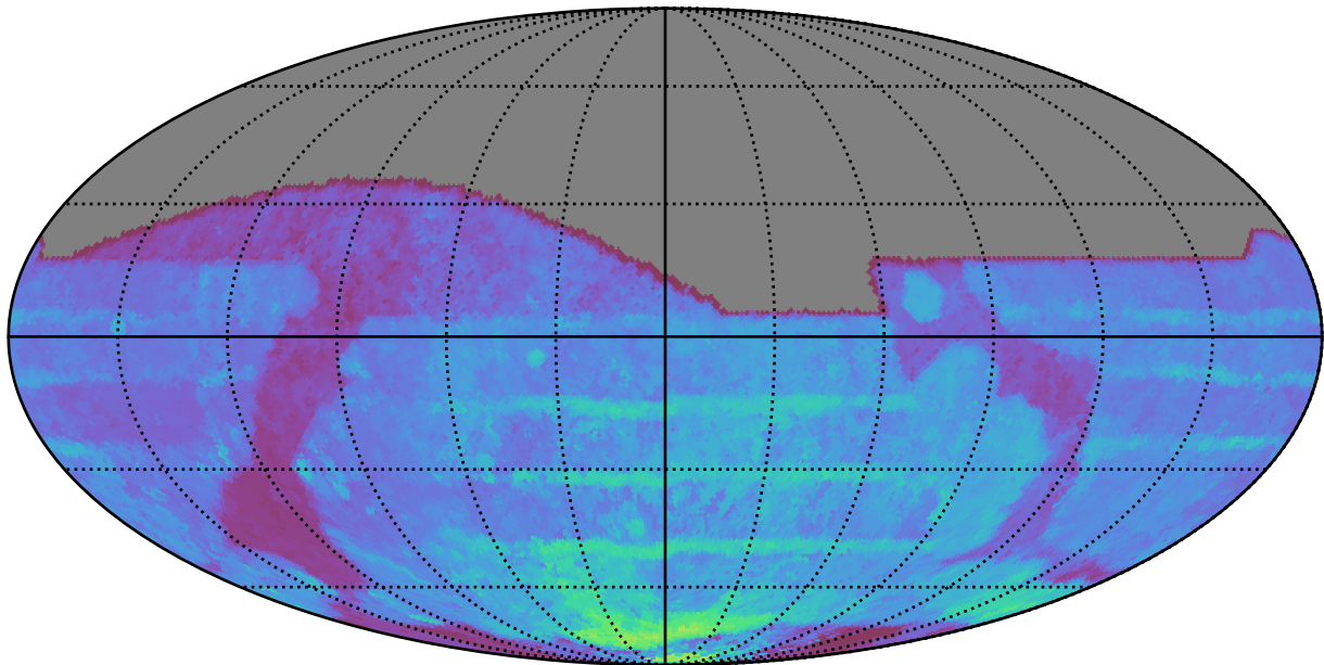
early_u_fpextra2.0_v3.4_10yrs All sky all bands: 80thPercentile Season Length
