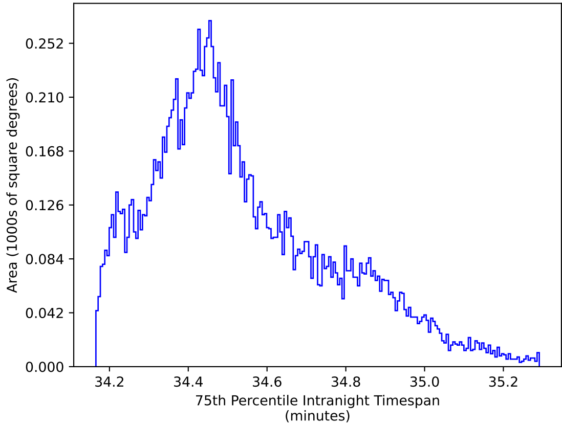
early_u_fpextra2.0_v3.4_10yrs WFD zy bands: 75th Percentile Intranight Timespan
