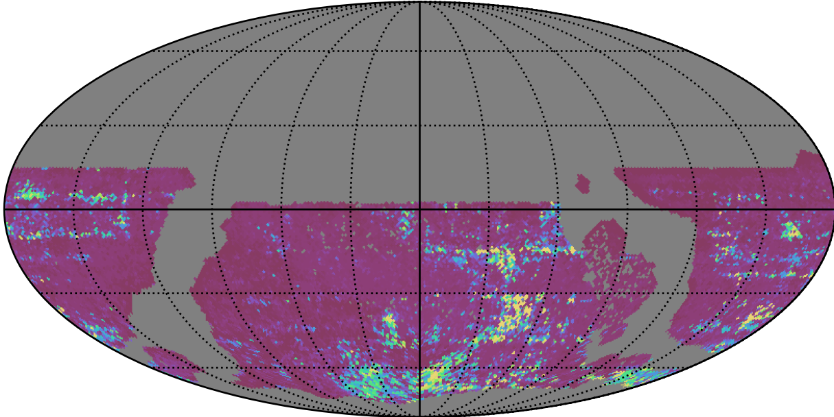
early_u_fpextra2.0_v3.4_10yrs WFD z band: 75th Percentile Intranight Timespan
