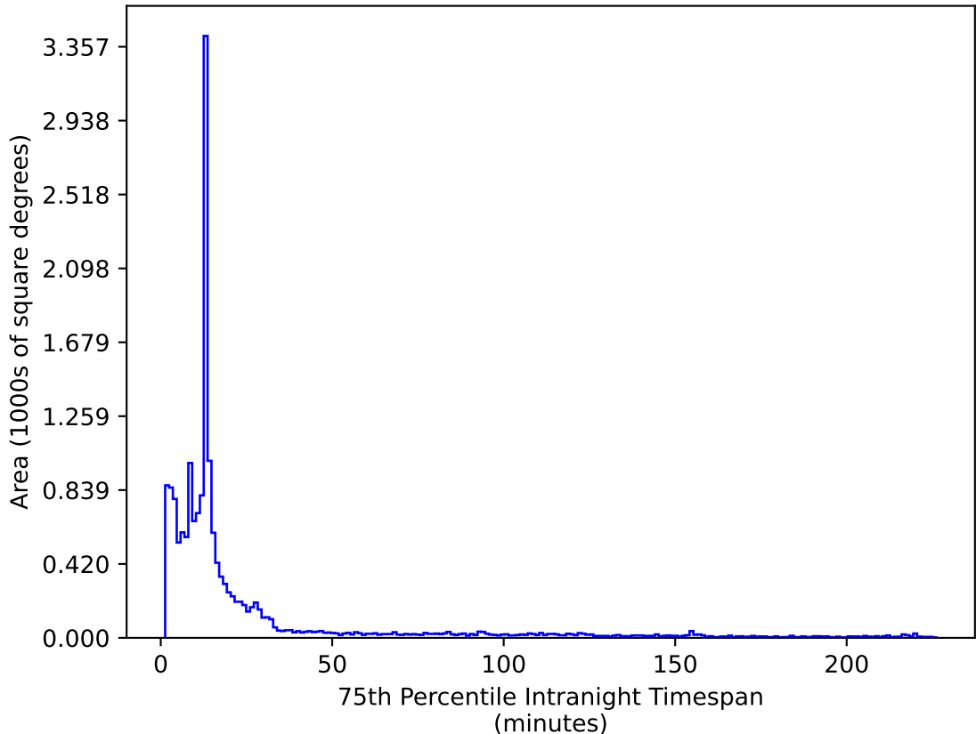
early_u_fpextra2.0_v3.4_10yrs WFD z band: 75th Percentile Intranight Timespan
