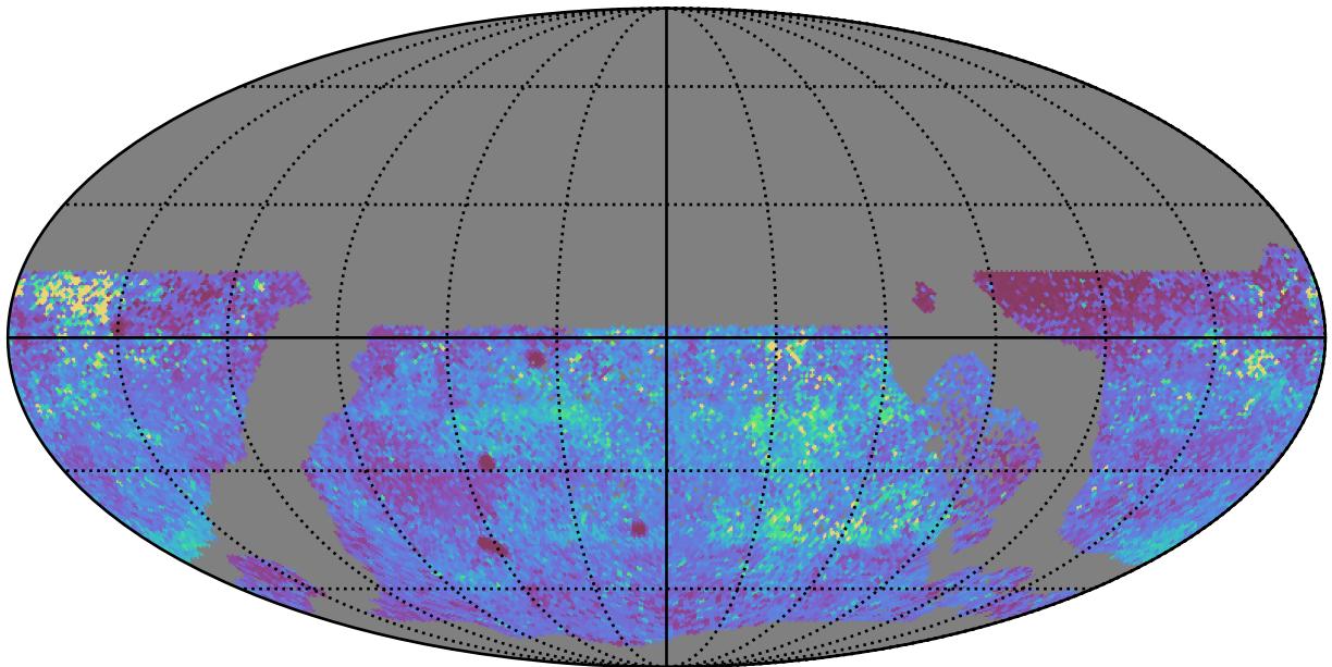
early_u_fpextra2.0_v3.4_10yrs WFD y band: 75th Percentile Intranight Timespan
