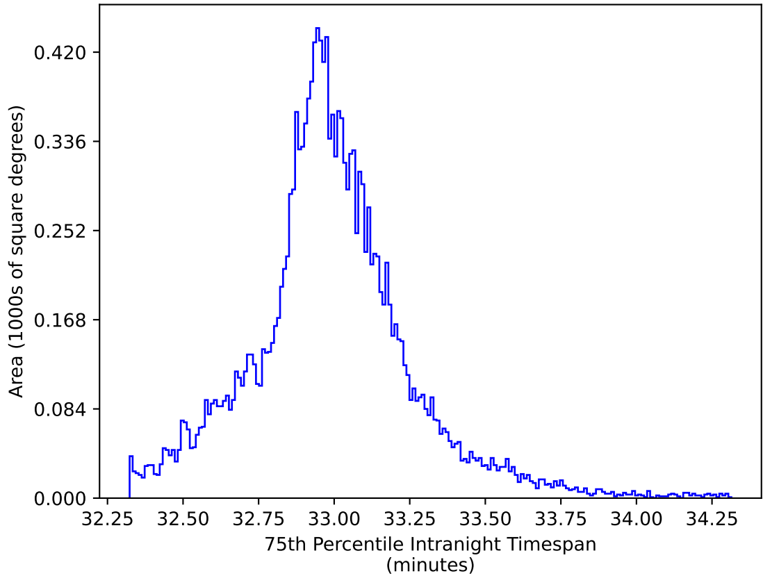
early_u_fpextra2.0_v3.4_10yrs WFD y band: 75th Percentile Intranight Timespan
