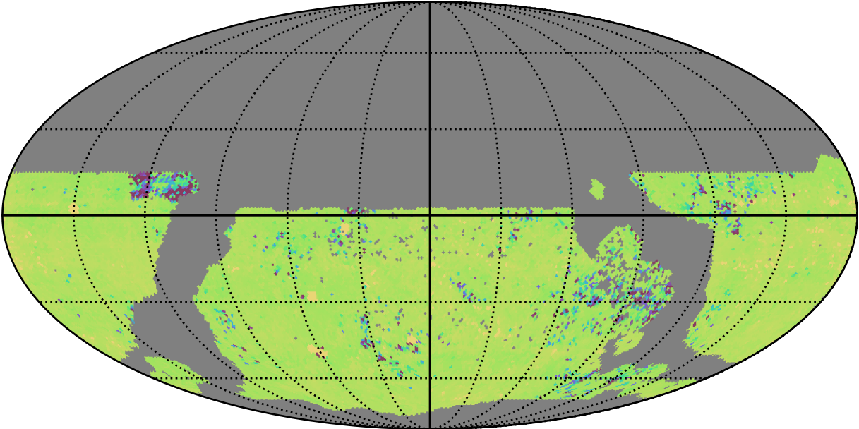
early_u_fpextra2.0_v3.4_10yrs WFD ug bands: 75th Percentile Intranight Timespan
