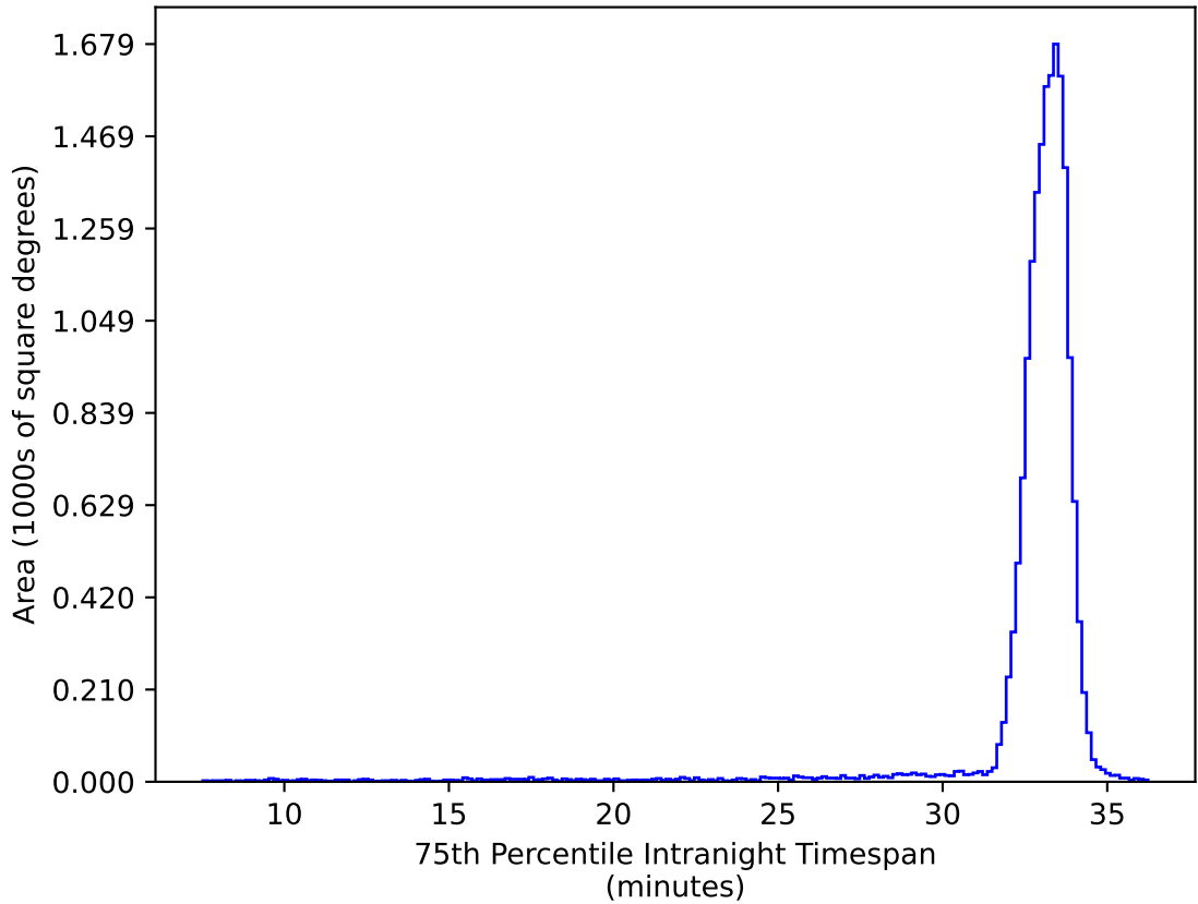
early_u_fpextra2.0_v3.4_10yrs WFD ug bands: 75th Percentile Intranight Timespan
