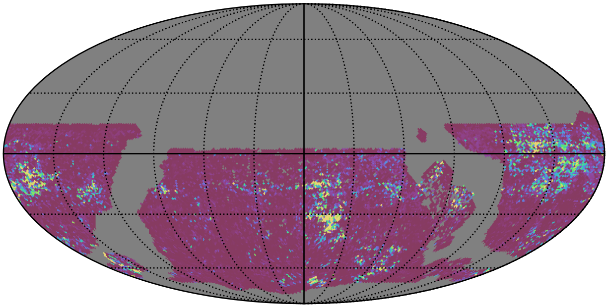
early_u_fpextra2.0_v3.4_10yrs WFD u band: 75th Percentile Intranight Timespan
