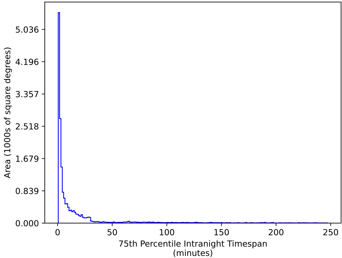
early_u_fpextra2.0_v3.4_10yrs WFD u band: 75th Percentile Intranight Timespan
