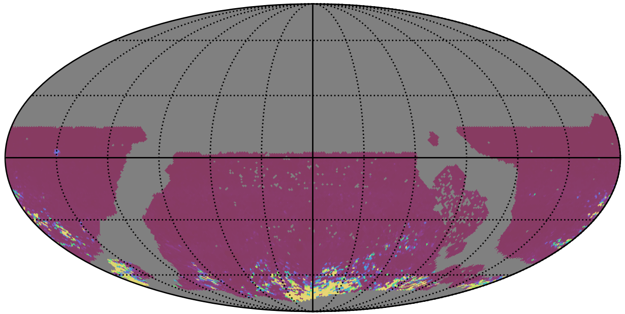
early_u_fpextra2.0_v3.4_10yrs WFD ri bands: 75th Percentile Intranight Timespan
