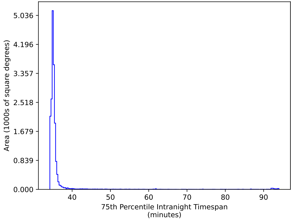
early_u_fpextra2.0_v3.4_10yrs WFD ri bands: 75th Percentile Intranight Timespan
