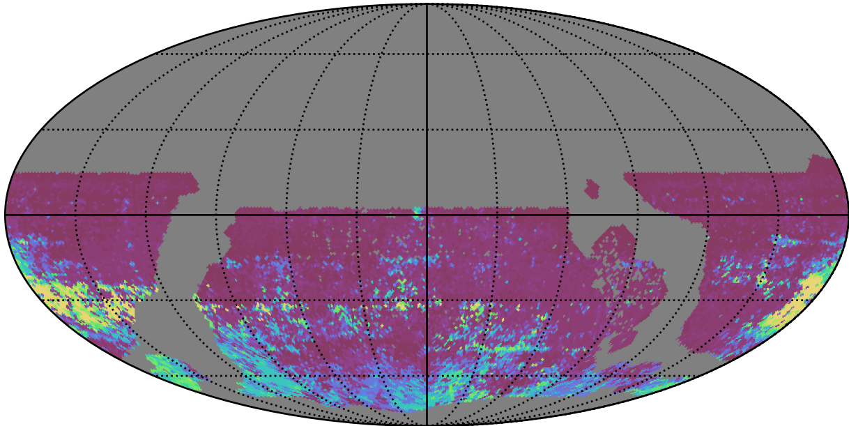
early_u_fpextra2.0_v3.4_10yrs WFD r band: 75th Percentile Intranight Timespan
