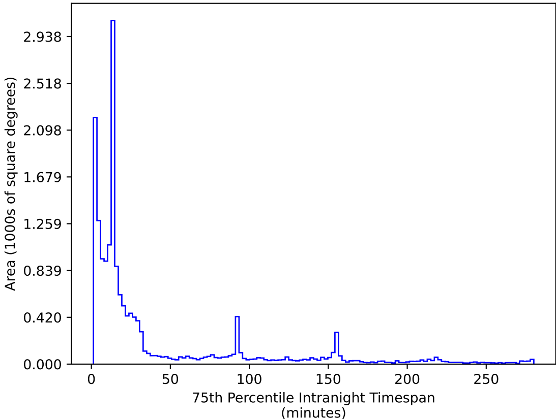
early_u_fpextra2.0_v3.4_10yrs WFD r band: 75th Percentile Intranight Timespan
