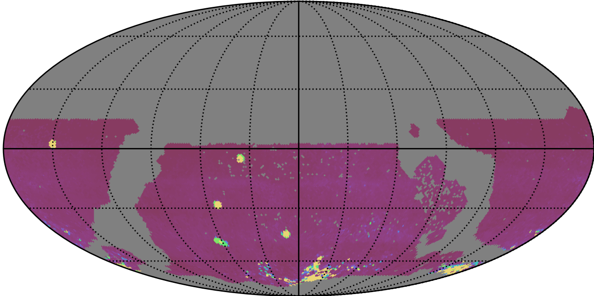
early_u_fpextra2.0_v3.4_10yrs WFD iz bands: 75th Percentile Intranight Timespan
