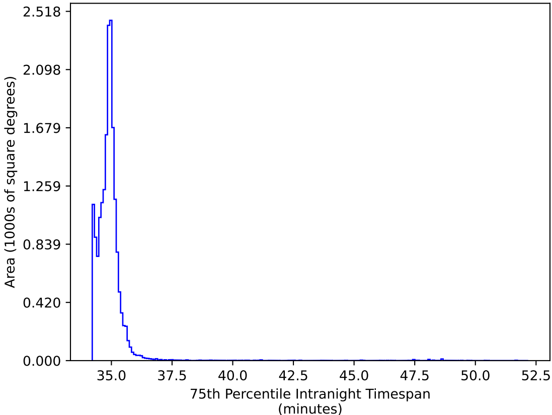
early_u_fpextra2.0_v3.4_10yrs WFD iz bands: 75th Percentile Intranight Timespan
