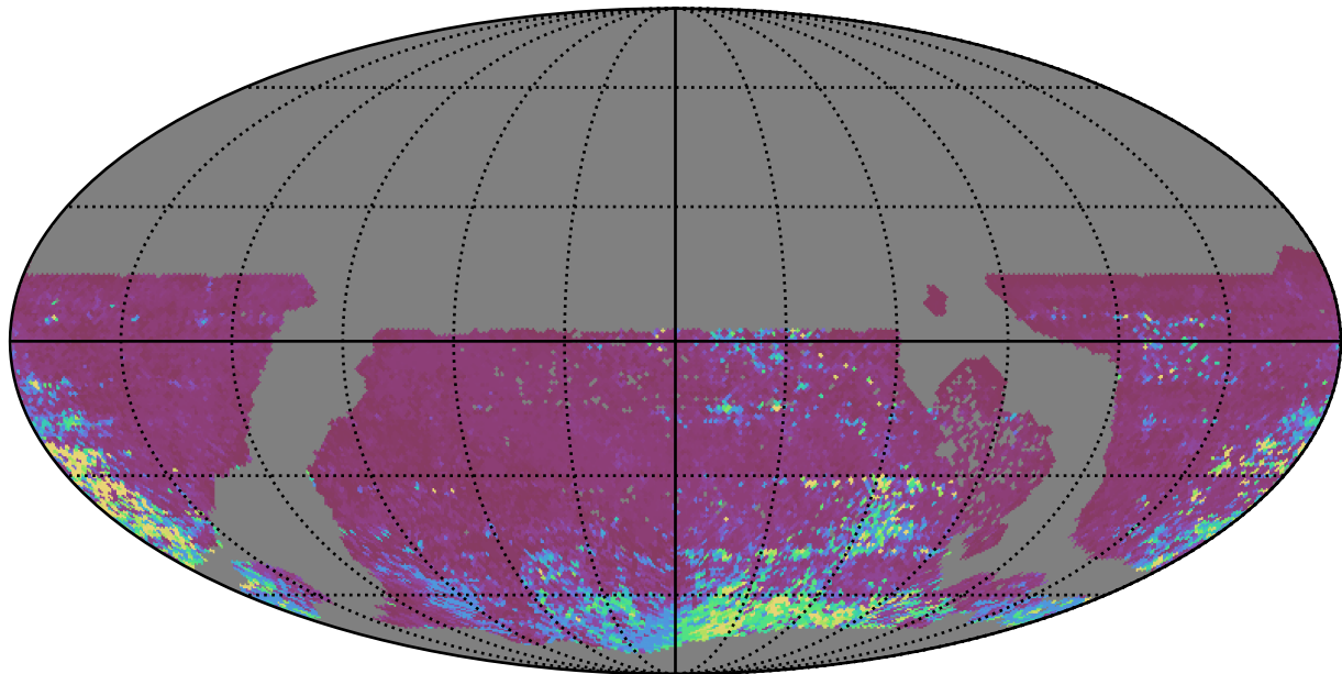
early_u_fpextra2.0_v3.4_10yrs WFD i band: 75th Percentile Intranight Timespan
