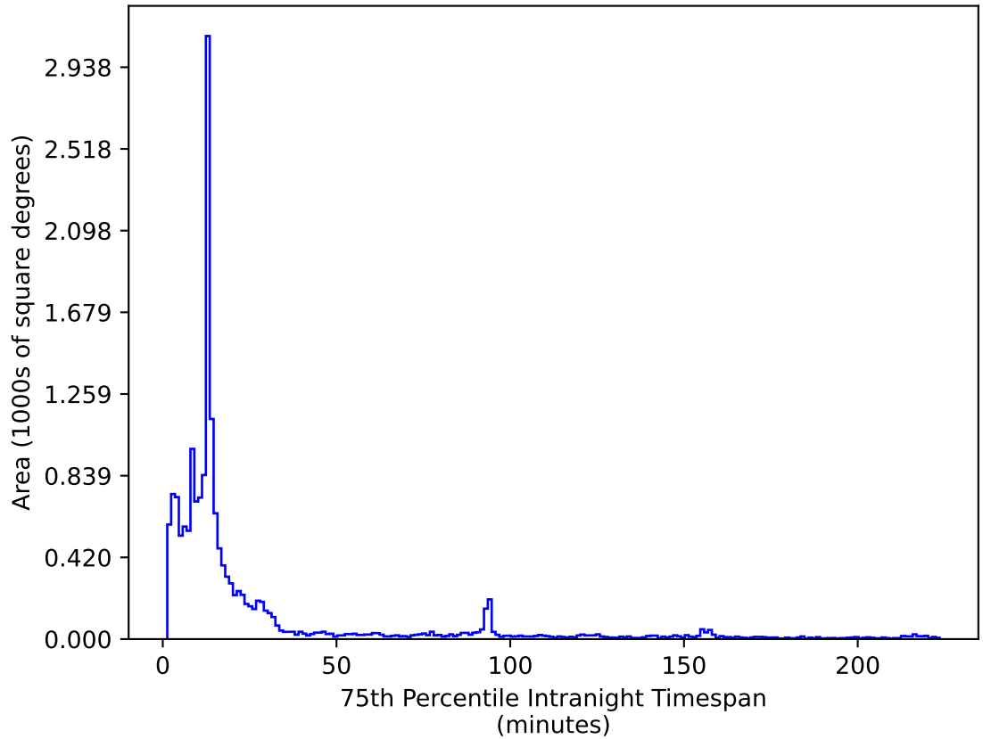
early_u_fpextra2.0_v3.4_10yrs WFD i band: 75th Percentile Intranight Timespan
