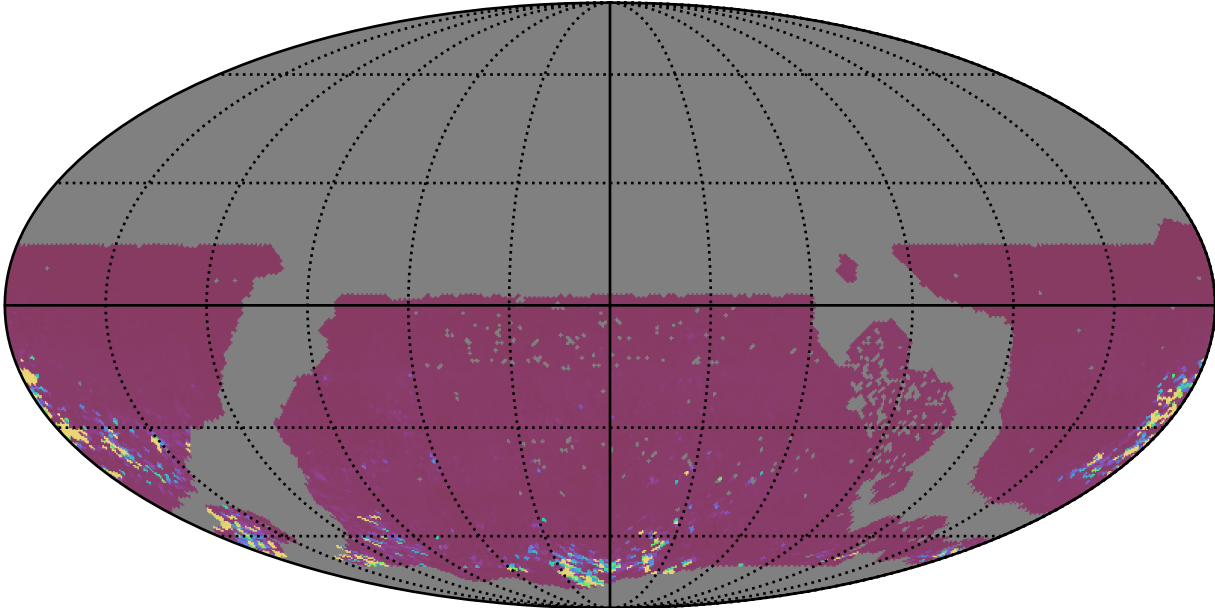
early_u_fpextra2.0_v3.4_10yrs WFD gr bands: 75th Percentile Intranight Timespan
