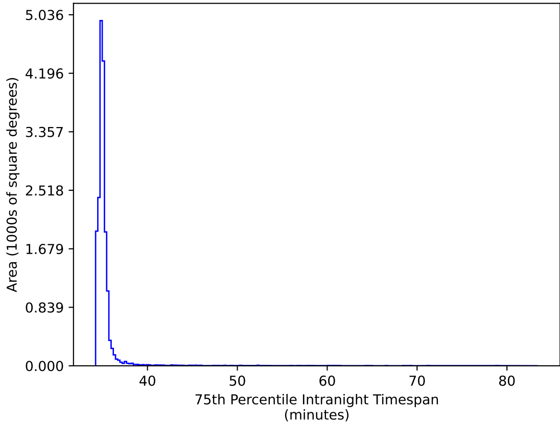
early_u_fpextra2.0_v3.4_10yrs WFD gr bands: 75th Percentile Intranight Timespan
