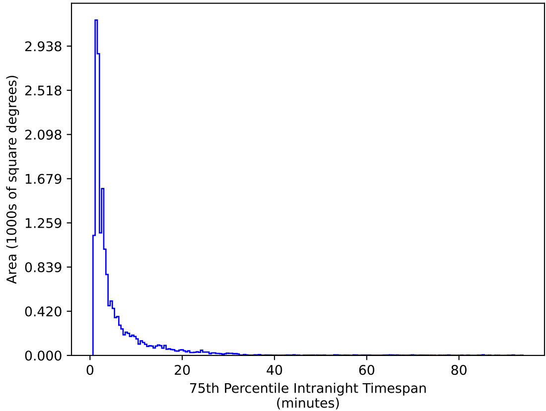
early_u_fpextra2.0_v3.4_10yrs WFD g band: 75th Percentile Intranight Timespan
