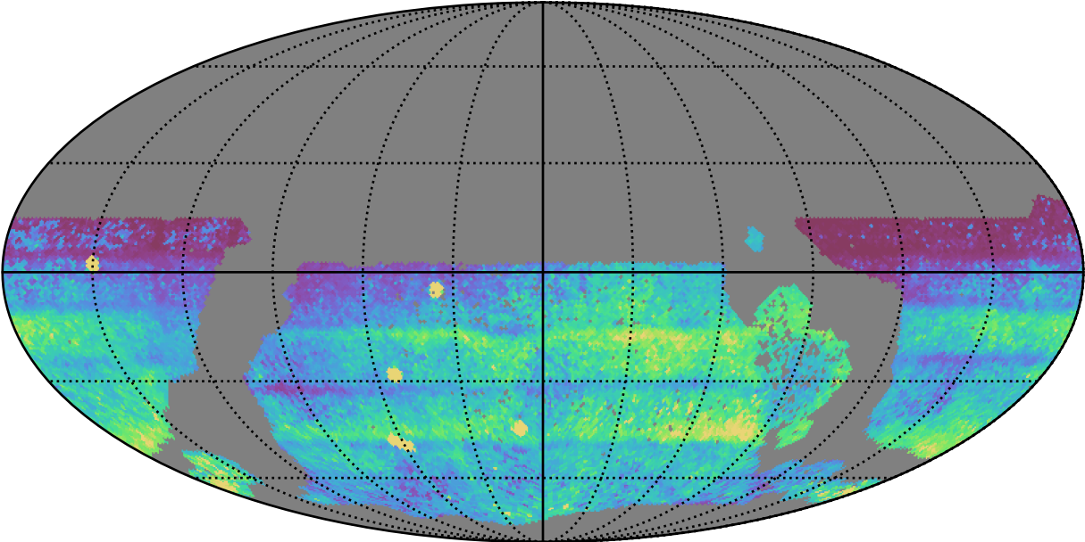
early_u_fpextra2.0_v3.4_10yrs WFD all bands: 75th Percentile Intranight Timespan
