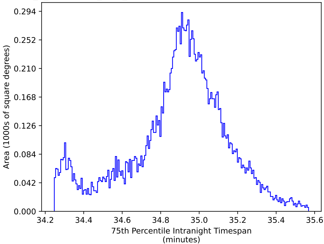
early_u_fpextra2.0_v3.4_10yrs WFD: 75th Percentile Intranight Timespan
