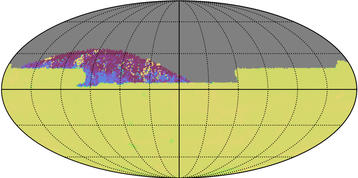
early_u_fpextra2.0_v3.4_10yrs All sky zy bands: 75th Percentile Intranight Timespan
