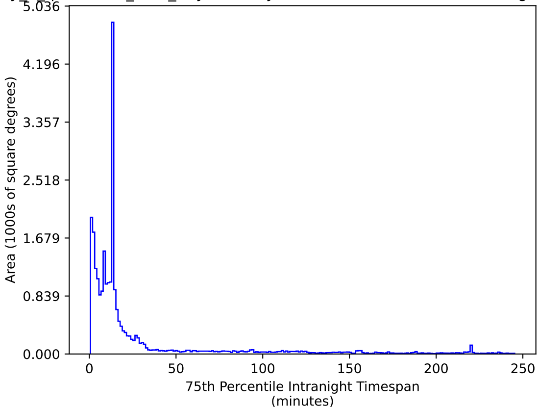
early_u_fpextra2.0_v3.4_10yrs All sky z band: 75th Percentile Intranight Timespan
