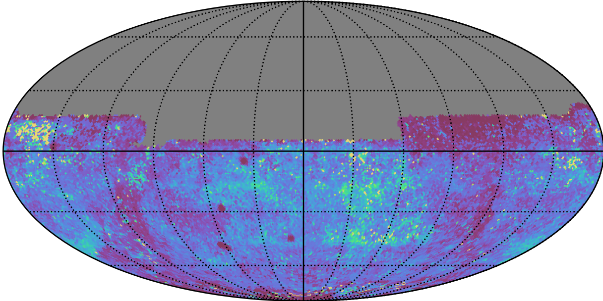
early_u_fpextra2.0_v3.4_10yrs All sky y band: 75th Percentile Intranight Timespan
