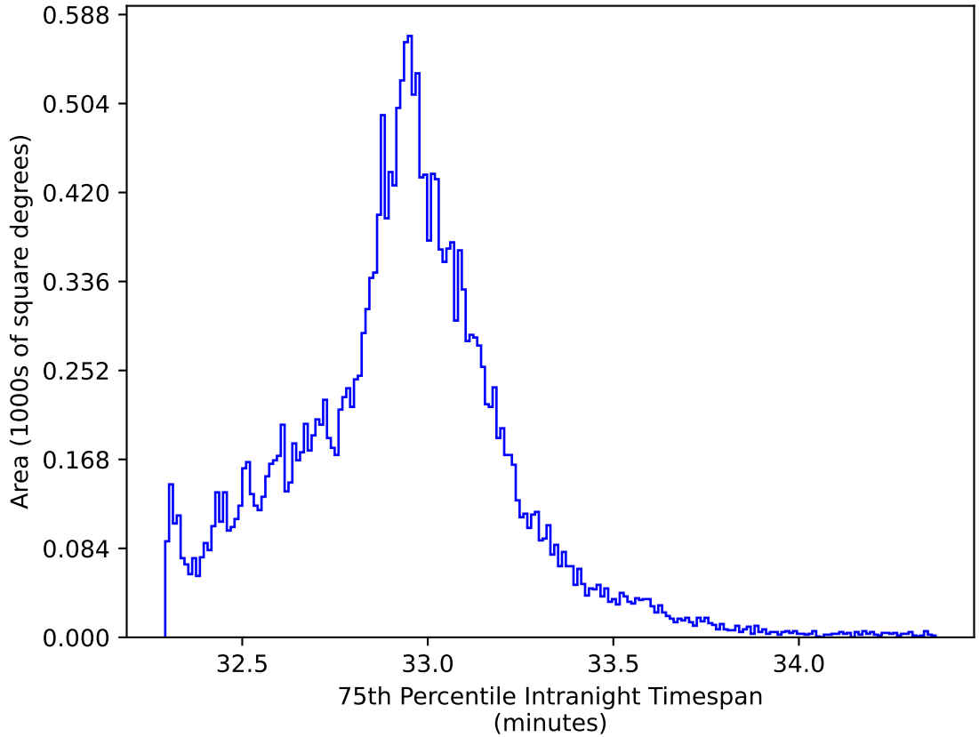
early_u_fpextra2.0_v3.4_10yrs All sky y band: 75th Percentile Intranight Timespan
