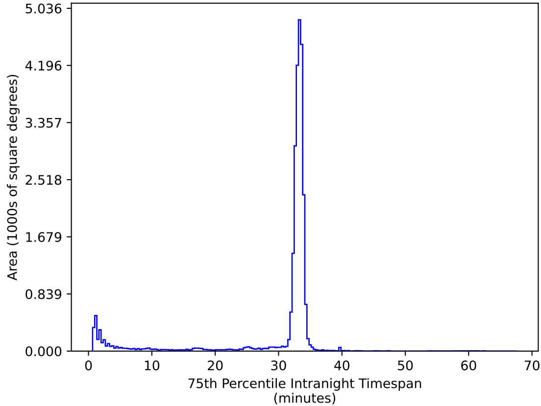
early_u_fpextra2.0_v3.4_10yrs All sky ug bands: 75th Percentile Intranight Timespan
