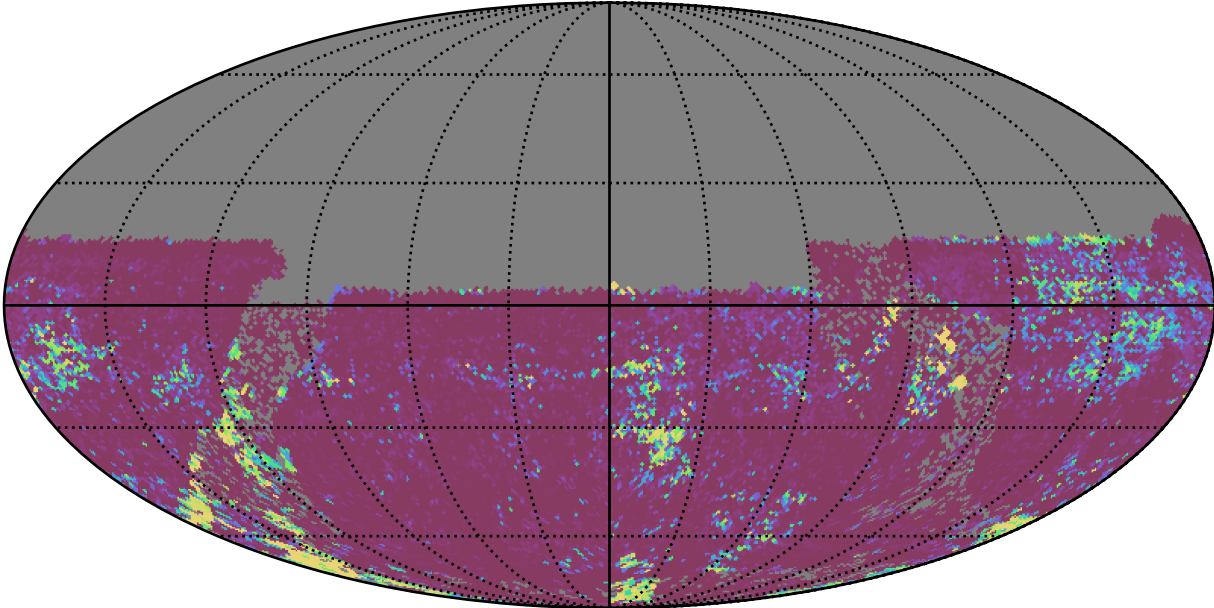
early_u_fpextra2.0_v3.4_10yrs All sky u band: 75th Percentile Intranight Timespan
