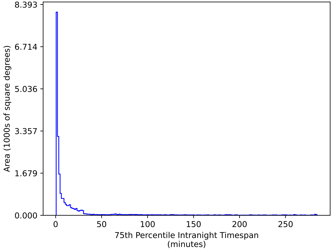
early_u_fpextra2.0_v3.4_10yrs All sky u band: 75th Percentile Intranight Timespan
