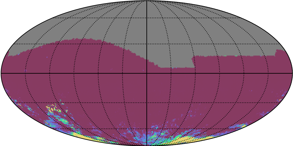
early_u_fpextra2.0_v3.4_10yrs All sky ri bands: 75th Percentile Intranight Timespan
