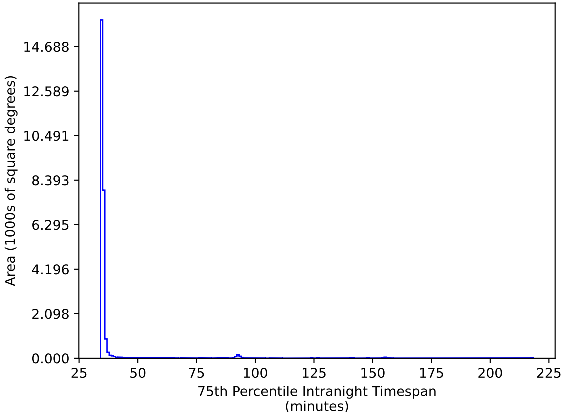
early_u_fpextra2.0_v3.4_10yrs All sky ri bands: 75th Percentile Intranight Timespan
