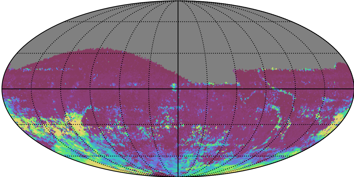
early_u_fpextra2.0_v3.4_10yrs All sky r band: 75th Percentile Intranight Timespan
